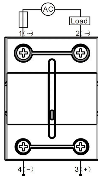
Wiring Diagram
