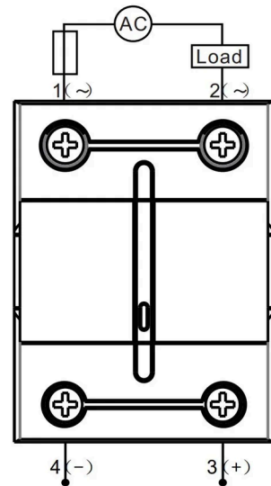
Wiring Diagram
