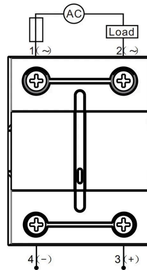
Wiring Diagram
